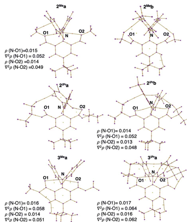
Fig. 3 Atom in molecules (AIM) analysis results based on X-ray geometries of 2^{\text{Me}}\mathbf{a-b} , 2^{\text{iPr}}\mathbf{a-b} , 3^{\text{Me}}\mathbf{a} and 3^{\text{iPr}}\mathbf{a} showing bond paths between the central nitrogen and the carbonyl oxygen, calculated at the RCAM- and UCAM-B3LYP-D3/def2-SVP levels in 2 and 3 , respectively.
