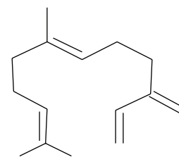
(E) - \beta -Farnesene
