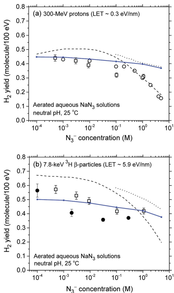
Fig. 3 Decrease in the molecular hydrogen yield (in molecule per 100 eV) with concentration of \text{N}_3^- ions for 300 MeV incident protons (LET \sim 0.3 eV \text{nm}^{-1} ) (panel a) and for 7.8 keV ^3\text{H} \beta -particles (LET \sim 5.9 eV \text{nm}^{-1} ) (panel b) in the radiolysis of air-saturated aqueous azide ( \text{NaN}_3 ) solutions (neutral pH, 25 ^\circ\text{C} ), calculated from our Monte Carlo simulations over the range of 10^{-4} to 5 M. The blue solid lines show our simulated results (see text). Experimental data for \gamma and tritium \beta -particle irradiations: ( \bullet ), ref. 22; ( \square ), ref. 25; ( \circ ), ref. 60. For the sake of comparison, the \text{H}_2 yields calculated from ref. 26 for both types of radiation, assuming that \text{N}_3^- scavenges the short-lived precursor to \text{H}_2 with a rate constant of 10^{12} \text{M}^{-1} \text{s}^{-1} (dashed line) and does not scavenge the short-lived precursor to \text{H}_2 (dotted line), are also shown in the figure.
