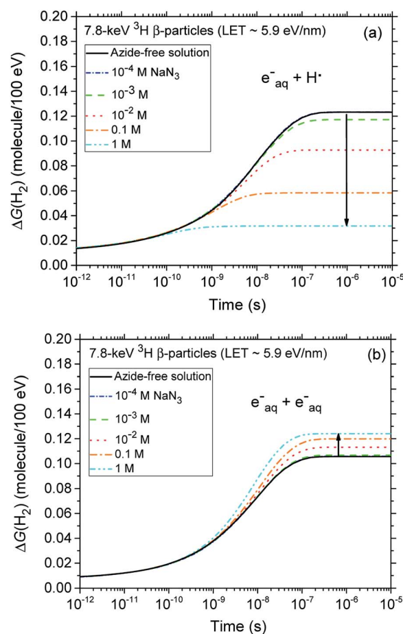
Fig. 4 Time dependence of the extents \Delta G(\text{H}_2) (in molecule/100 eV) of the reactions ( e_{\text{aq}}^- + \text{H}^* ) (panel a) and ( e_{\text{aq}}^- + e_{\text{aq}}^- ) (panel b) that contribute to the formation of molecular hydrogen, calculated from our Monte Carlo simulations of the radiolysis of air-saturated aqueous azide ( \text{NaN}_3 ) solutions (pH neutral, 25 ^\circ\text{C} ) by 7.8 keV ^3\text{H} \beta -particles (LET \sim 5.9 eV \text{nm}^{-1} ) in the time interval 1 ps to 10 \mu\text{s} . The blue, green, red, orange, and cyan lines correspond to the five different concentrations of azide anions studied: 10^{-4} , 10^{-3} , 10^{-2} , 0.1, and 1 M, respectively (see text). For the sake of reference, the black lines in panels a and b show the cumulative yield variations \Delta G(\text{H}_2) of the two reactions ( e_{\text{aq}}^- + \text{H}^* ) and ( e_{\text{aq}}^- + e_{\text{aq}}^- ) that contribute to the formation of \text{H}_2 in azide-free solutions. Finally, the concentration of dissolved oxygen used in the simulations was 2.5 \times 10^{-4} M.
