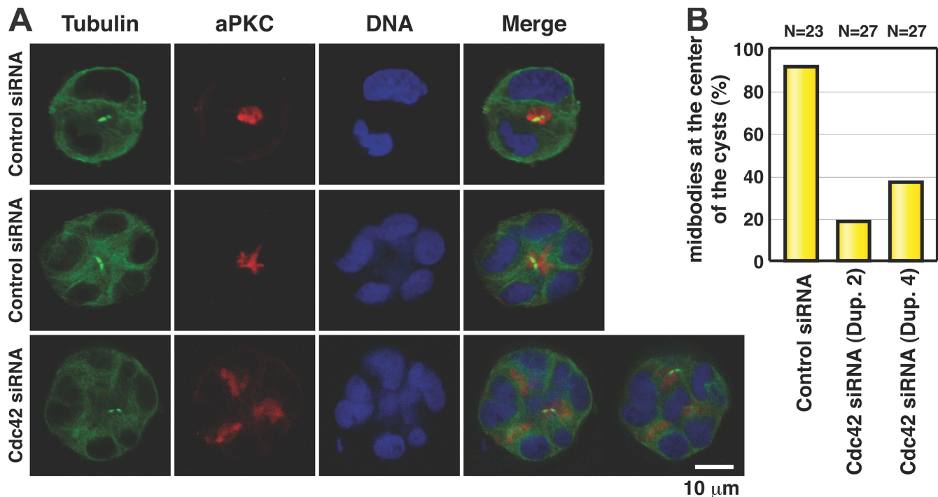
Figure 5. The midbody positions the apical surface during cyst development. (A) Caco-2 transfected with control or Cdc42 siRNA was fixed and stained for DNA (blue), tubulin (green), and aPKC (red). (top) A control cyst at the two-cell stage (note that abscission appears to have occurred symmetrically). (middle) A larger control cyst, with the midbody in the center of the developing structure (apical region of dividing cell) reflecting asymmetric abscission. (bottom) Cdc42 siRNA structure with one midbody positioned normally at the center and another midbody (located in a different z section) abnormally positioned. (B) Quantitation of midbodies at the center of the cyst from three independent experiments. The total number of midbodies is indicated (N). A midbody is regarded as being in the center if it is located at a distance from the centroid that is less than one third the radius of the structure.
