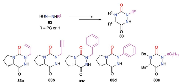
Scheme 29 Substituents variation at position 2.
