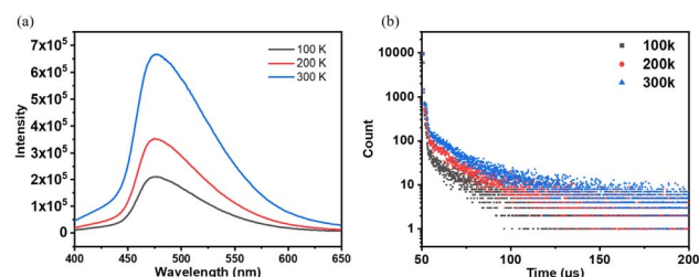
Fig. 3 (a) Fluorescence spectrum and (b) fluorescence intensity decay curve of the solid state of NI-mPCz at different temperatures.
