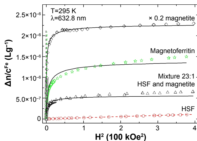
Figure 12 Reduced linear magnetic birefringence.
