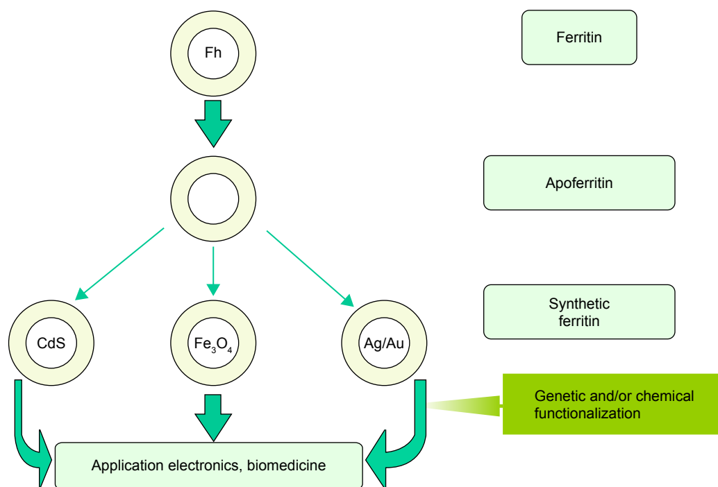
Figure 10 Schematic representation of synthetic pathway.
