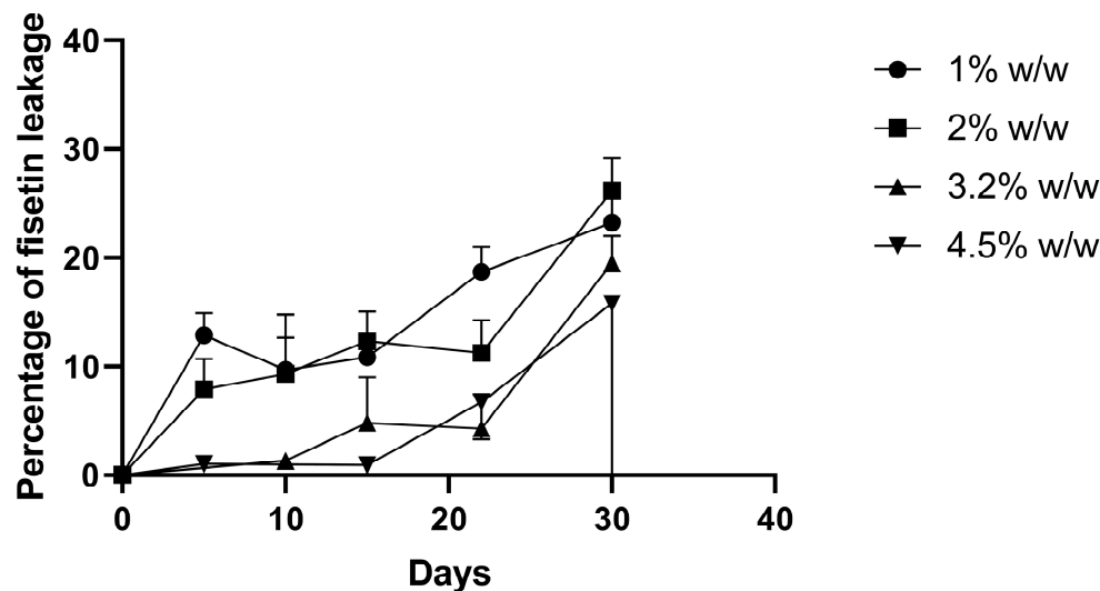
Figure 3. Stability of fisetin-loaded liposomes F4 containing 1, 2, 3.2 or 4.5 wt% of cholesterol (mean \pm SD, n = 2). Liposomes were purified using filtration to remove non-encapsulated and precipitated fisetin at each sampling time.
