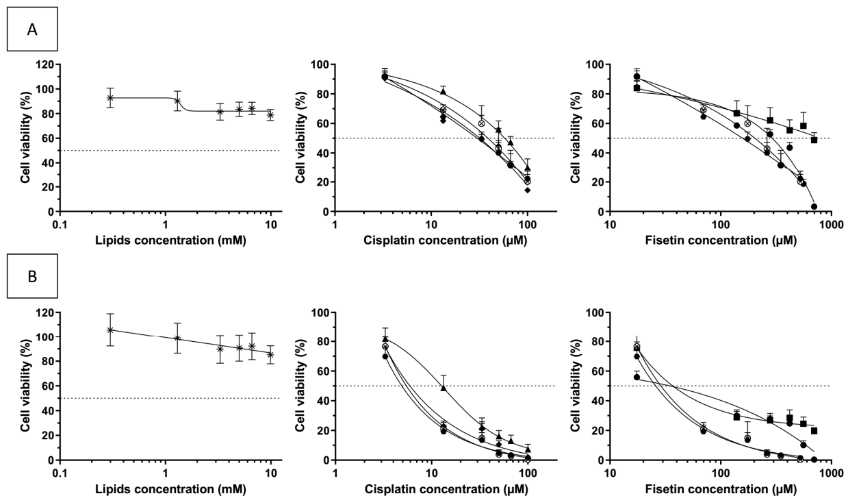
Figure 7. Comparison of the cytotoxicity of empty liposomes (star), free fisetin (circle), free cisplatin (diamond), fisetin-loaded liposomes (square), cisplatin-loaded liposomes (triangle), mixture of fisetin-loaded liposomes and cisplatin-loaded liposomes (cross in circle) and liposomes co-encapsulating fisetin and cisplatin (hexagone) after 24 h (A) or 48 h (B) of exposure (mean \pm SD, n = 5 ).
