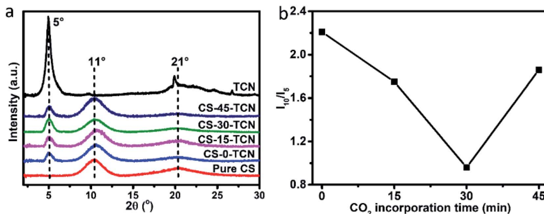
Fig. 5 (a) XRD patterns of TCN, CS and CS/TCN composites; (b) intensity ratio of 10^\circ and 5^\circ .
