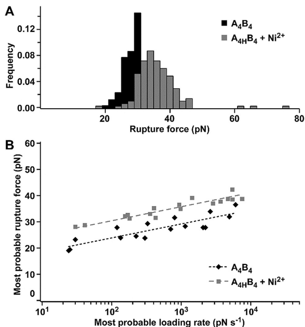
Figure 4. AFM-based SMFS of the \text{His-Ni}^{2+} -His stapled coiled coil in PIPPS-BS. A) Rupture force histogram (retract speed 400 \text{ nm s}^{-1} ). B) Dynamic SMFS data ( n=3 ) fitted to the Bell-Evans model (dashed lines). \text{Ni}^{2+} : \geq 500 \mu\text{M NiCl}_2 .
