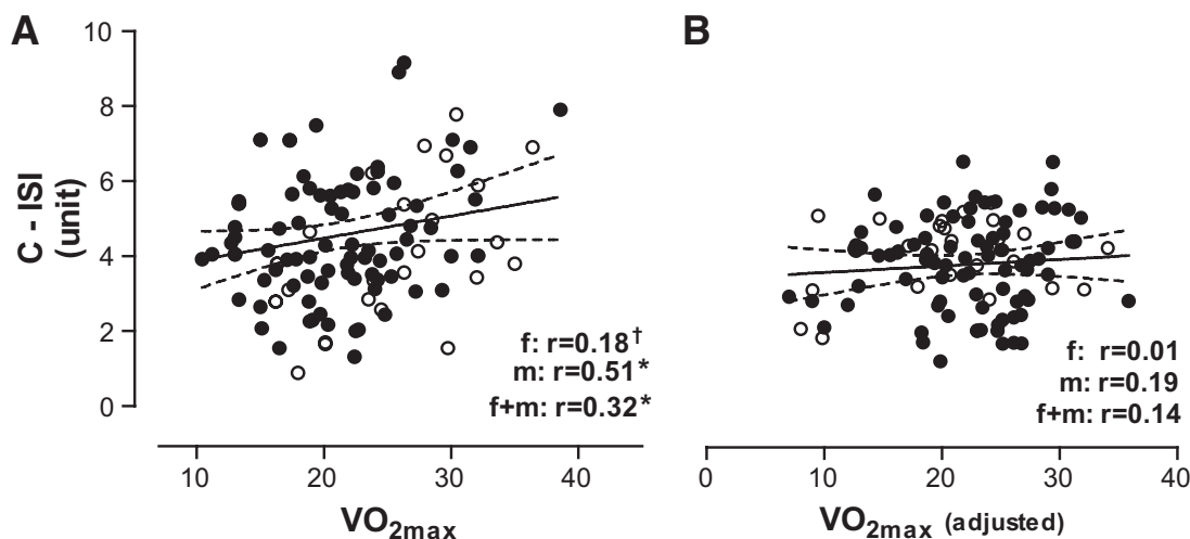
FIG. 1. Correlation between C-ISI and VO_{2max} before (A: r = 0.32 , P < 0.05 ) and after adjustment for intrahepatic lipid content (B: r = 0.14 , NS); ●, women; ○, men. * P < 0.05 ; † P < 0.1 and >0.05 .
