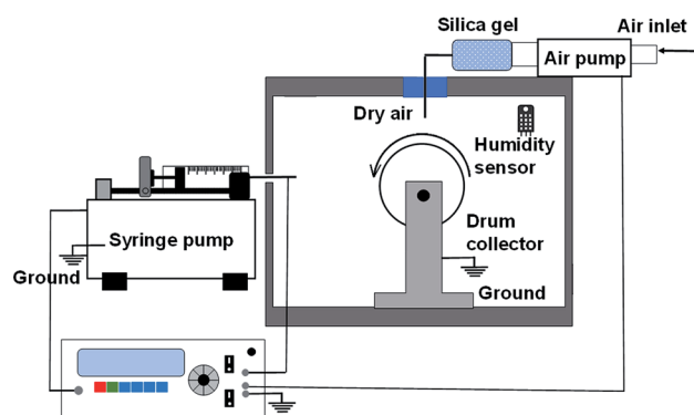
Fig. 1 Schematic diagram of the electrospinning apparatus.
