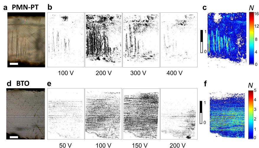
Fig. 1 Localization of avalanches for PMN-PT and BTO. Optical image of the initial state of the sample for a PMN-PT and d BTO. The scale bar indicates 200 \mu\text{m} . Switched regions for b PMN-PT and e BTO, at representative applied voltages. The black regions (assigned to 1) are regions that switched between t and t + \delta t , with \delta t = 1/30 s, while the white regions (assigned to 0) remained unchanged. Accumulated activity maps after a full hysteresis loop for c PMN-PT and f BTO. The colour scale indicates the number of times each pixel ( \sim 1 \mu\text{m}^2 in size) has been changed.
