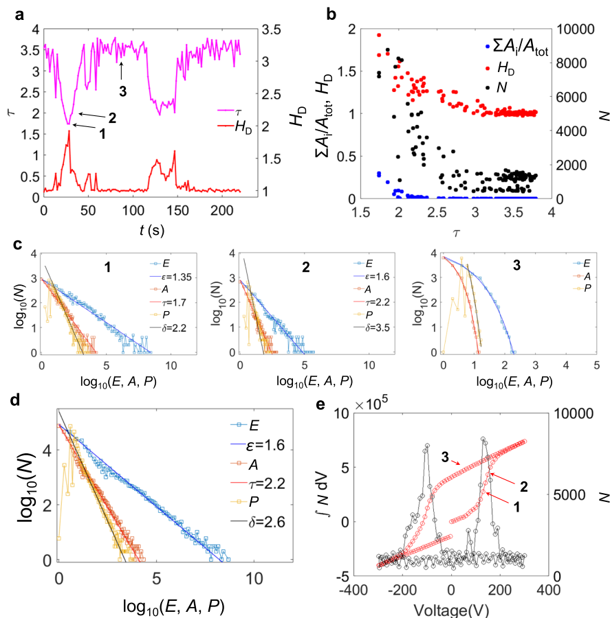
Fig. 4 Scale-invariant avalanches in BTO. a H_D and \tau as a function of time. b H_D , \Sigma A_i/A_{\text{tot}} (proportion of switched regions with respect to the total area) and N (avalanche activity, defined as the number of switched regions between t and t + \delta t ) as a function of \tau . c E (energy), A (area) and P (perimeter) distribution at the time steps marked as 1, 2 and 3 by arrows in a . d E , A and P distribution from all the time steps. e N as a function of the applied voltage (right axis) and its integration over the voltage applied (left axis).
