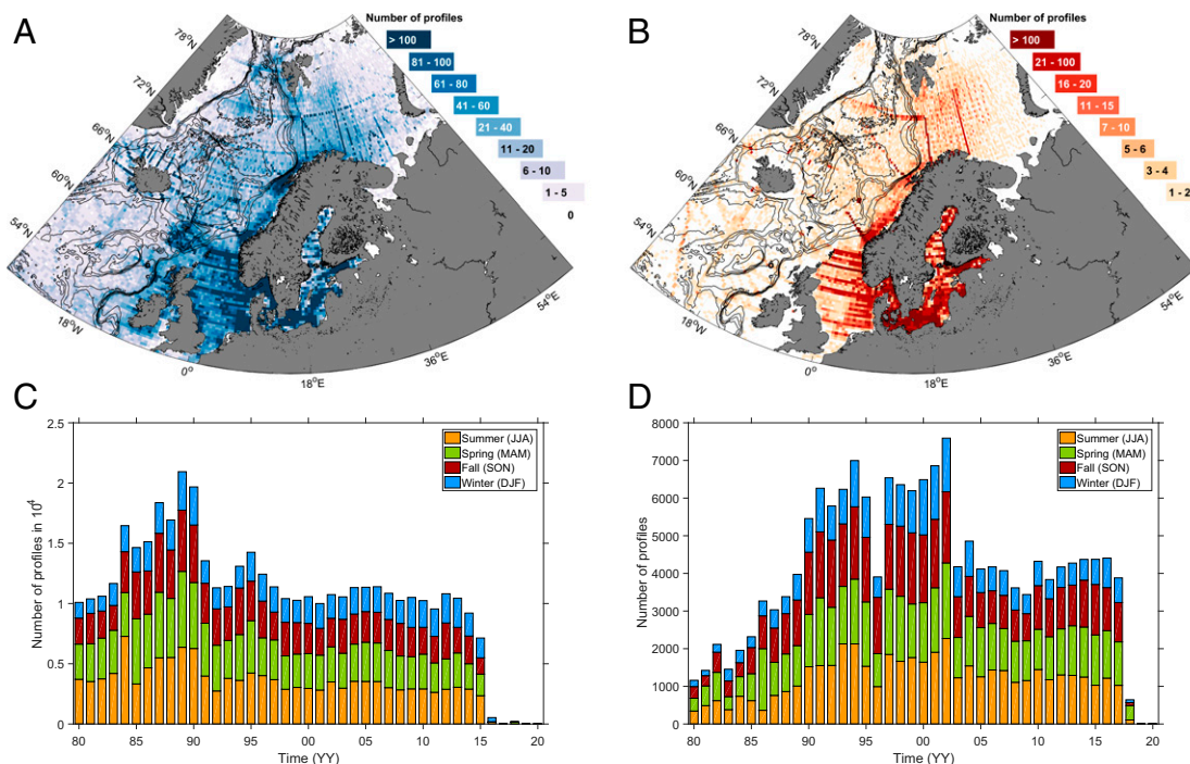
Fig. 1. Data distribution of ( A and C ) temperature/salinity and ( B and D ) nutrients/oxygen. ( A and B ) Total number of vertical profiles per 0.5^\circ longitude \times 0.25^\circ latitude bin since 1980. ( C and D ) Number of vertical profiles per year, color coded by season. Note the different scales. The data were obtained from Unified Database for Arctic and Subarctic Hydrography, ICES, World Ocean Database, the international Argo program, Global Ocean Data Analysis Project version 2, Institute of Marine Research (Norway), Marine and Freshwater Research Institute of Iceland, and the Norwegian Iceland Seas Experiment database. Duplicates between the archives have been discarded. Note the asymmetry in spatial data, with high coverage in the eastern part of the basin where current change is least and vice versa. There is a considerable seasonal bias in data available from the seas neighboring the Nordic countries, with highest density for spring and summer, a feature prone to impact our understanding of past as well as future changes. JJA, June, July, August; MAM, March, April, May; SON, September, October, November; DJF, December, January, February.
