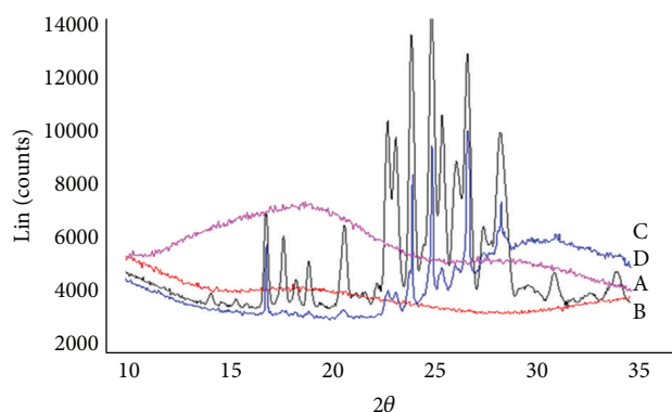
FIGURE 8: Overlay of XRPD pattern of A. free CUR; B. HPMCAS-HF; C. physical mixture; and D. optimized formulation (P5).
