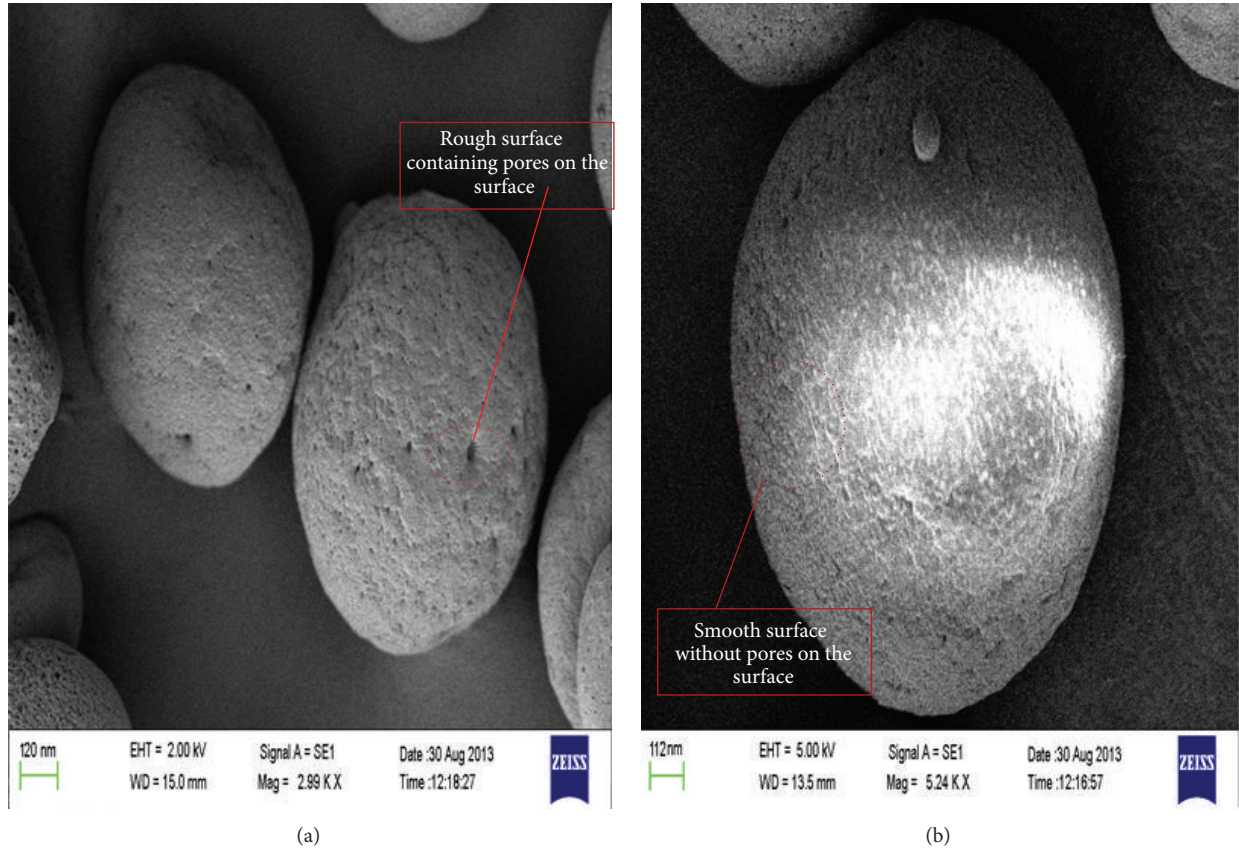
FIGURE 9: Scanning electron microscopy (SEM) images of optimized formulation (P5) without plasticizer (a) and optimized formulation (P5) with plasticizer (b).
