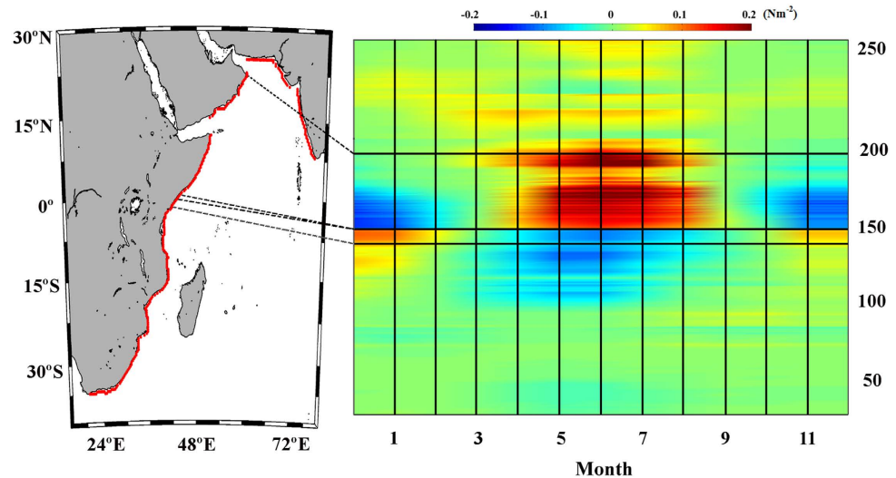
Figure 9. Wind stress along the Western Indian Ocean. Annual cycle of alongshore wind stress ( \text{Nm}^{-2} ) for the period 1982–2010. Red points on the map show the coastal points analysed. Black lines indicate those regions considered to be coastal upwelling areas. This figure has been performed using Matlab.
