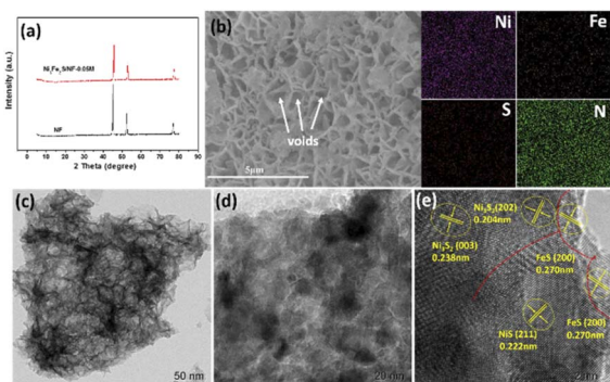
Fig. 2 (a) XRD patterns of the samples, (b) SEM images and the corresponding mapping of \text{Ni}_6\text{Fe}_2\text{S}/\text{NF}-0.05\text{ M} collected on SEM, (c and d) TEM images and (e) HR-TEM image of \text{Ni}_6\text{Fe}_2\text{S}/\text{NF}-0.05\text{ M} .
