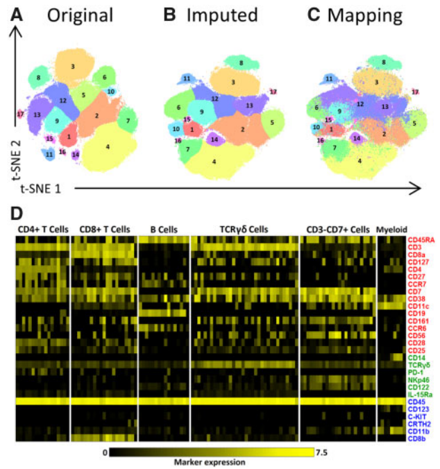
Fig. 3. Clustering of the original and the imputed datasets. (A–C) t-SNE maps showing the different identified populations in the CD4+T Cells lineage. (A) Shows the populations of the original data. (B) The populations of the imputed data (for m = 16 , L1 = 6 and L2 = 6 ). (C) The mapping of the original clusters labels on the t-SNE map of the imputed data. (D) Heatmap of markers expression for the 121 characterized immune cells populations of the original dataset for m = 16 . Black-to-yellow scale shows the median arcsinh-5 transformed values for the markers expression. Markers colors indicate whether a marker is shared between panels or unique to a single panel, during panels combination (red is shared, green is unique to panel A, blue is unique to panel B)
