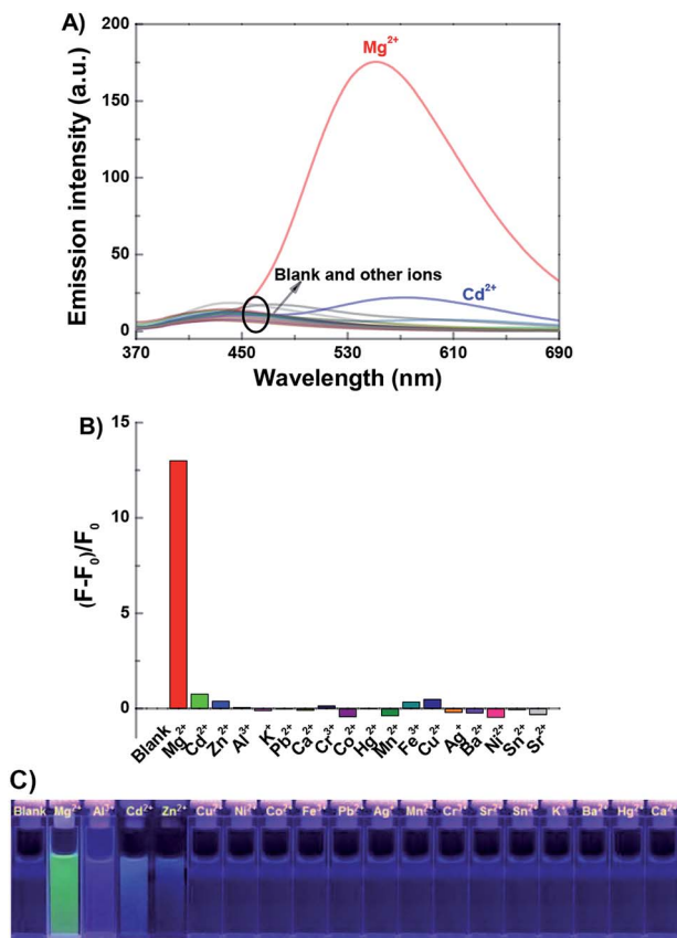
Fig. 2 Upon addition various metal ions to 1o ( 2.0 \times 10^{-5} mol L ^{-1} in acetonitrile): (A) fluorescence emission spectral changes; (B) emission intensity changes; (C) fluorescent photos ( \lambda_{\text{ex}} = 350 nm).
