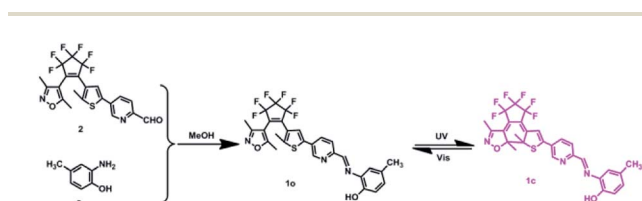
Scheme 1 The synthetic route and photochromism of 1o .
