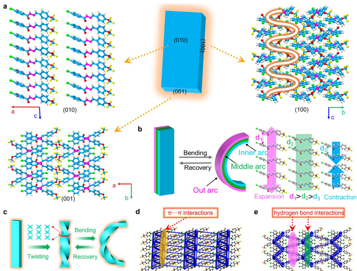
Fig. 6 Structural basis of the mechanical deformation of CTBB crystals. (a) Molecular packing of form I viewed perpendicular to the (001), (010), and (100) planes. (b) Schematic of the mechanism for the elastic bending of CTBB crystals. (c) Schematic showing the mechanism of plastic twisting of form I. (d and e) Energy frameworks of form I shown together with the \pi\cdots\pi (d) and hydrogen bonding (e) interactions. The pink and green envelopes represent intermolecular interactions related to the \pi -stacked columns along different directions.
