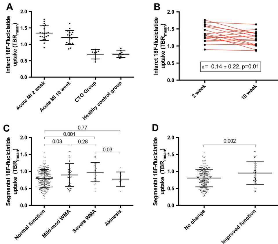
Figure 4 ^{18}\text{F} -Fluciclatide uptake in myocardial infarction (MI) is shown. Uptake of ^{18}\text{F} -fluciclatide in (A) patients with acute MI at 2 and 10 weeks, patients with chronic total occlusion and healthy control subjects is shown. Uptake was greatest at 2 weeks after MI (B). ^{18}\text{F} -Fluciclatide uptake in the acute MI group was greater in regions of hypokinesia when compared with sites of normal function or akinesis (C). This translated to a higher ^{18}\text{F} -fluciclatide uptake in those regions which subsequently improved in function on follow-up cardiac magnetic resonance (D). CTO, chronic total occlusion; TBR, tissue-to-background ratio. WMA, wall motion abnormality.
