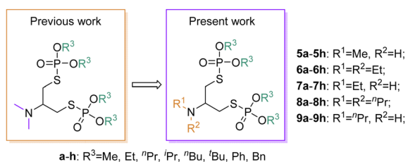
Fig. 2 The structures of target compounds.
