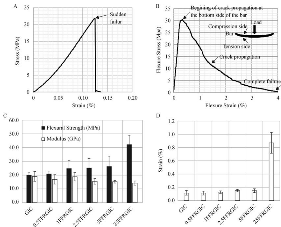
Fig. 3 Flexural properties. Stress-strain curves of (A) Ketac TM Fil Plus and (B) 5wt% flax fibers-reinforced GIC as obtained from the three-point bending test as an example to show the ductile behavior of fibers-reinforced formulations with 5 and 25wt. % fibers content. The inset represent the compression and tension side of the bar under three-point bending; the failure normally starts at the tension (bottom) side (C) Flexure strength (MPa) and modulus (GPa). (D) Flexure strain (%) of Ketac TM Fil Plus and flax fibers-reinforced Ketac TM Fil Plus. Bars represent mean ( n = 6 ) while error bars represent standard deviations. * refers to statistical significance from Ketac TM Fil Plus. The significance level was set at 0.05.
