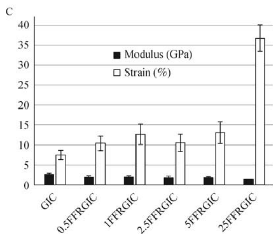
Fig. 2 Compressive properties. A: Stress-strain curves obtained from the compression test, B: compressive (MPa) and yield strength (MPa), C: compressive modulus (GPa) and strain (%) of Ketac™ Fil Plus and flax fibers-reinforced Ketac™ Fil Plus. Bars represent mean ( n = 6 ) while error bars represent standard deviations. * refers to statistical significance from Ketac™ Fil Plus. The significance level was set at 0.05.
