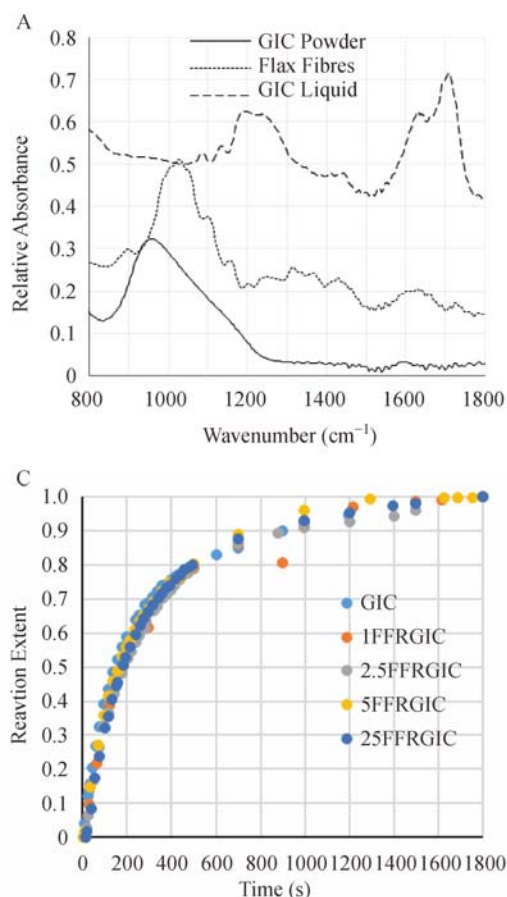
Fig. 1 Starting components and setting reaction. A: FTIR spectra of the starting components of flax fiber modified Ketac™ Fil Plus restorative glass ionomer. B: Difference spectra, obtained by subtracting the initial absorbance from the final absorbance, for 2.5FFRGIC as an example. C: Reaction extent versus time, measured using the peak at 1565\text{ cm}^{-1} , of Ketac™ Fil Plus and flax fibers reinforced Ketac™ Fil Plus.
