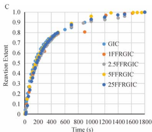
Fig. 1 Starting components and setting reaction. A: FTIR spectra of the starting components of flax fiber modified Ketac™ Fil Plus restorative glass ionomer. B: Difference spectra, obtained by subtracting the initial absorbance from the final absorbance, for 2.5FFRGIC as an example. C: Reaction extent versus time, measured using the peak at 1565\text{ cm}^{-1} , of Ketac™ Fil Plus and flax fibers reinforced Ketac™ Fil Plus.
