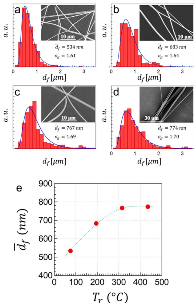
Fig. 10 Diameter distribution for different T_r : (a) 75 ^\circ\text{C} , (b) 195 ^\circ\text{C} , (c) 315 ^\circ\text{C} , and (d) 435 ^\circ\text{C} . d_f represents the geometric mean diameter and \sigma_g is the geometric standard deviation. (e) Fibers' geometric mean diameter as a function of real furnace temperature, T_r (the green dotted line is to guide the eye only).
