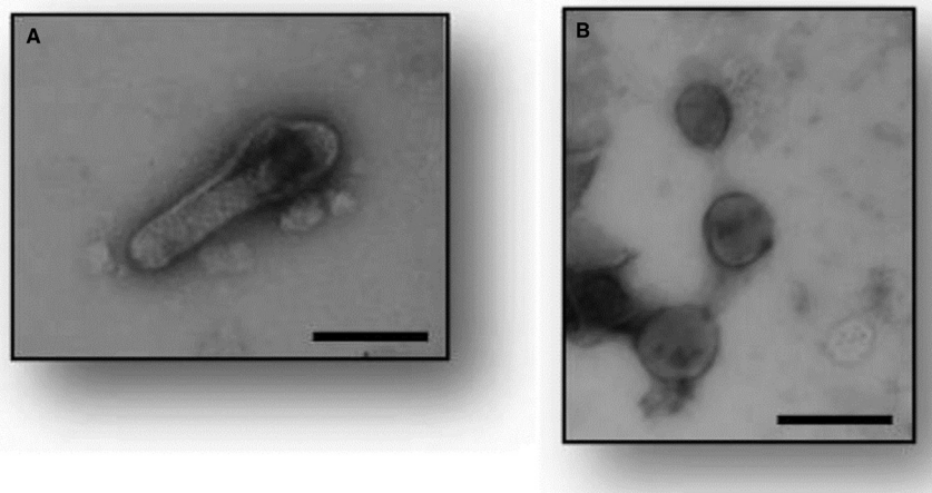
Fig. 1 Electron micrographs of negatively stained (A) Autographa californica multicapsid nucleopolyhedrovirus and (B) retrovirus. Scale=100 nm.
