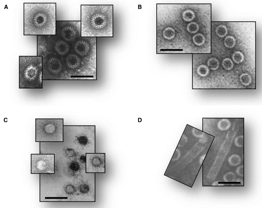
Fig. 2 Electron micrographs of negatively stained rotavirus-like particles: (A) triple-layered 2/6/7 particles; (B) double-layered 2/6 particles; (C) single-layered VP2 particles; and (D) VP6 tubes [79]. Scale=100 nm.
