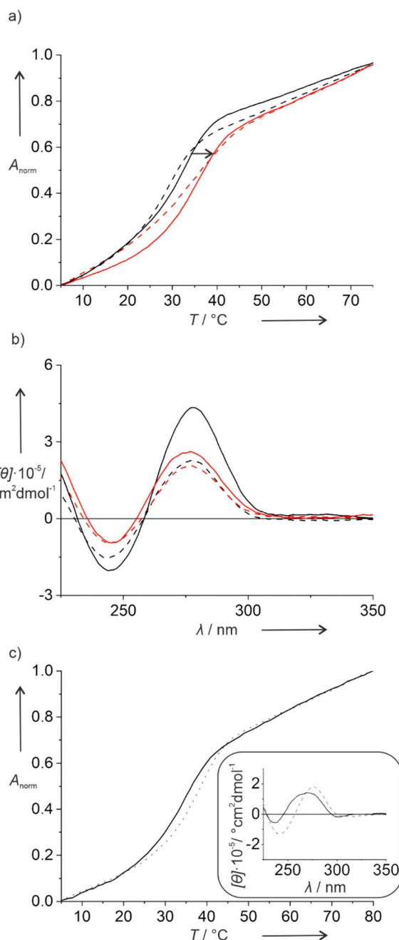
Fig. 1 (a) Melting curves and (b) CD spectra of duplexes \text{III}^{\text{Tri,GNA}} , \text{III}^{\text{PtCN,GNA}} , \text{III}^{\text{Tri,DNA}} and \text{III}^{\text{PtCN,DNA}} . Broken lines represent the use of the GNA linker, solid lines of the DNA linker. Data for PtCN -containing DNA are shown in red, for the Pt(II)-free reference strands in black. (c) Melting curves of duplexes \text{I}^{\text{PtCN,DNA}} (dotted line) and V (solid line). The inset shows the corresponding CD spectra. Experimental conditions: 1 \mu\text{M} DNA duplex, 5 mM MOPS buffer (pH 7.0), 150 mM \text{NaClO}_4 , 2.5 mM \text{Mg}(\text{ClO}_4)_2 .
