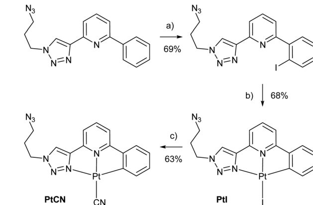
Scheme 1 Synthesis of the Pt(II) precursor complexes PtI and PtCN for the subsequent cycloaddition to a suitably alkyne-modified oligonucleotide. (a) NIS, Pd(OAc) 2 , CH 3 CN, 90 °C, 2 d; (b) Pt 2 (dba) 3 , THF, 50 °C, 90 min; (c) KCN, CH 3 OH/CH 3 CN (1 : 1), 90 °C, 3 h. For further synthetic details, see ESI.†
