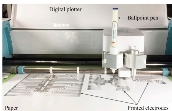
Figure 1. Printing setup for patterning electrode arrays on paper for the fabrication of a digital microfluidic (DMF) chip by using a ballpoint pen and a digital plotter.
