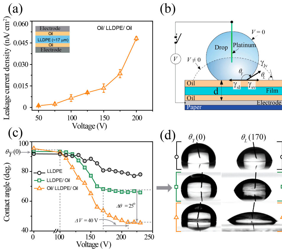
Figure 4. (a) Leakage current density across the LLDPE-dielectric film and its schematic measurement (inset). Characterization of the electrowetting on dielectric (EWOD) experiment on the LLDPE-dielectric film: (b) EWOD setup, and (c,d) the electro-spreading of the drop under applied voltages.
