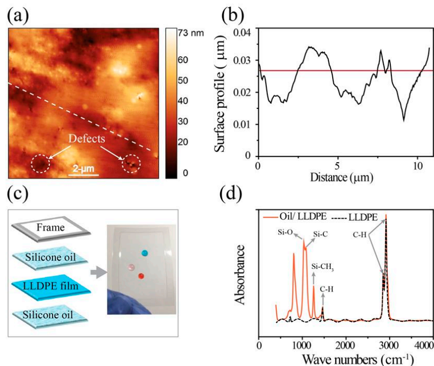
Figure 3. Surface morphology of the commercial LLDPE film. (a) Atomic force microscopy (AFM) image of the film and (b) representative surface profile extracted from (a) at the dashed line. (c) Schematic structure of a dielectric film prepared for the paper-based DMF chip and a photograph of the prepared dielectric film with three colorful drops on it. (d) FT-IR spectrum of a LLDPE-dielectric film with and without a silicone oil coated.
