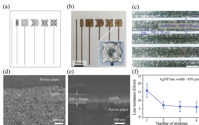
Figure 2. Printing silver nanoparticle (AgNP) electrodes on paper. (a) Electrode designs with various sizes and shapes, (b) electrodes printed with the designs in (a) and (inset) an enlargement of one design, and (c) printed AgNP lines. SEM images of the printed pattern: (d) top view and (e) cross-sectional view. (f) Surface electrical resistance of the printed AgNP line versus the number of printings.
