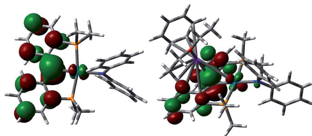
Fig. 5 HOMO for [\{\text{PC}(\text{sp}^2)\text{P}^{\text{tBu}}\text{PdNPh}_2\}]^- (5', left) and [\{\text{PC}(\text{sp}^2)\text{K}(\text{OEt}_2)(\text{C}_6\text{H}_6)\text{P}^{\text{tBu}}\text{PdNPh}_2\}] (5'', right).
