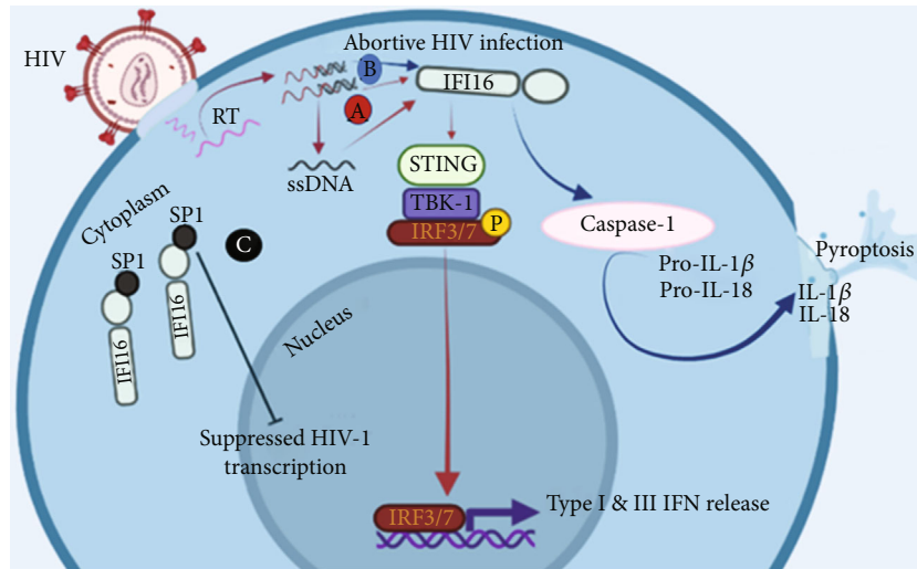
FIGURE 2: An illustration of the various mechanisms and pathways triggered by activated IFI16 in an HIV infection. (A) The activation of the STING-TBK1-IRF3/7 pathway by IFI16 after the sensing of retroviral DNA intermediates or ssDNA. (B) The activation of the IFI16 inflammasome and resulting cell death due to the accumulation of incomplete DNA reverse transcripts of HIV during an abortive HIV infection. (C) Restriction of HIV-1 replication by IFI16 independently of immune sensing through the binding and inhibition of the host transcription factor Sp1.
