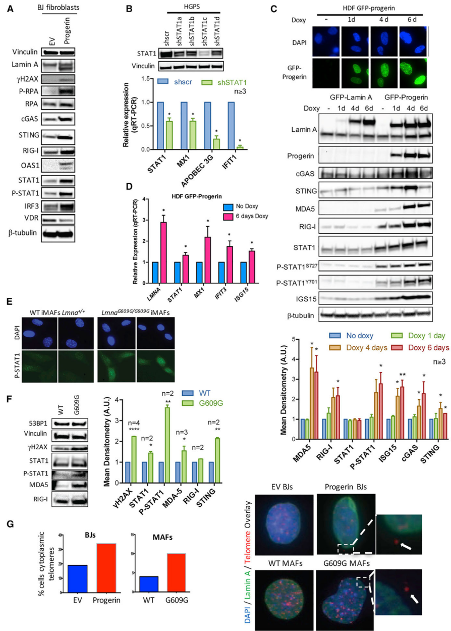
Figure 3. Activation of PRRs, STAT1, and ISGs by Progerin
