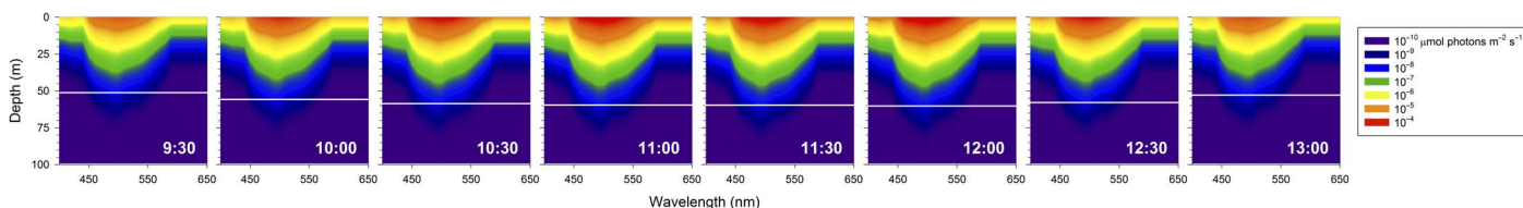
Fig. 3. Modeled depth of a constant light level (isolume) set to be the depth limit of copepod light-mediated behavior in Kongsfjorden. Underwater spectral scalar irradiance [ E_o(\lambda) , \mu\text{mol photons m}^{-2} \text{s}^{-1} ] was weighted by the spectral response of C. finmarchicus to yield a photometric quantity of Calanus -utilized light that is shown in colored contours as a function of depth at 30-min intervals on the 23 January Jetyak deployment. White horizontal lines show the depth of an isolume at 5 \times 10^{-8} \mu\text{mol photons m}^{-2} \text{s}^{-1} of Calanus -utilized light. UTC, coordinated universal time.
