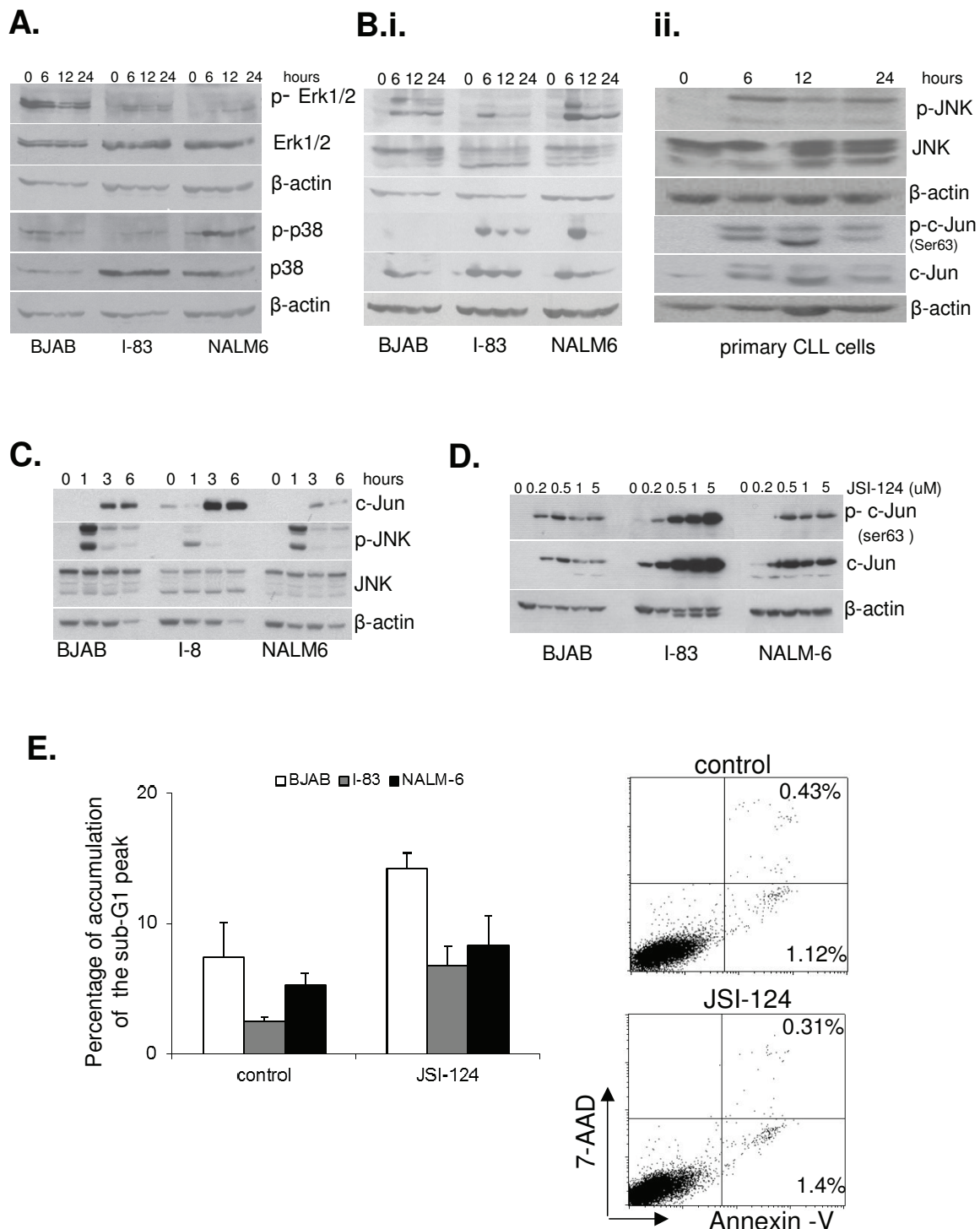
Figure 1 JSI-124 induces phosphorylation of c-Jun in B-leukemia cells. A, and B. I-83, BJAB, NALM-6 cells were treated with 1 μM JSI-124 for a 6 and 24 hour time course. Cell lysates were used for immunoblotting for the presence of p-JNK/JNK, p-p38/p38, p-p42/44 and p42/44 and p-c-Jun/c-Jun. Experiments were done at least in triplicate for all cells and for primary CLL cells. Representative original data are shown in Fig.1. C. All three cell lines were treated with 1 μM JSI-124 for 6 hours. D. Cells were treated with various doses of JSI-124 for 6 hours. Phospho- and total c-Jun levels were assessed by immunoblotting. E. BJAB, I-83, and NALM-6 cells were treated with 0.2 μM concentration of JSI-124 for 24 hour. Apoptosis was measured using flow cytometric analysis for accumulation of sub-G1 phase (upper panel) or Annexin V/7AAD staining. Data represents 3 independent experiments. Standard error was determined on the basis of three independent experiments.
