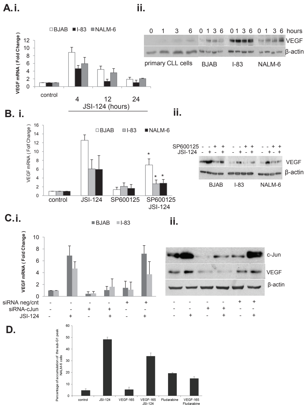
Figure 4 JSI-124 induced VEGF via activation of c-Jun. A. Increased levels of VEGF protein were detected by western blotting and mRNA by real time PCR in I-83, BJAB, NALM-6 cells after treatment with JSI-124 for the indicated times. Representative original data from four independent experiments are shown. B. BJAB, I-83 and NALM-6 cells were pretreated with 20 μmole/ml SP600125 for 1 hour following JSI-124 treatment for additional 4 hours. VEGF mRNA and protein levels were detected by RT-PCR and western blotting, respectively. Standard error was determined on the basis of three independent experiments and an asterisk represents significant difference (a p value of < 0.05) between JSI-124 alone or pretreated with SP600125. C. in BJAB and I-83 cells c-Jun was knocked down by using siRNA for c-Jun or non-target control siRNA. Total RNA was extracted and real time-PCR was used to detect mRNA level of VEGF. Error bars represent the standard errors for three independent experiments. Cell extract was assayed for western blotting for VEGF. Knock-down of c-Jun was confirmed by western blotting with antibody to c-Jun. D. NALM-6 cells were treated with 20 ng/ml VEGF-165 for 1 h and followed by JSI-124 for 24 h. The percentages of apoptotic cells were determined by FACS analysis for sub-G1 accumulation.
