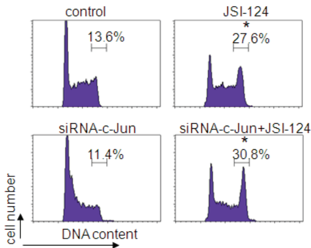
Figure 3 JSI-124 mediated c-Jun activation was not dependent on STAT3 expression in B-cell leukemia. A and B, Cells were transfected with siRNA-STAT or siRNA-c-Jun or siRNA non-target control. Then cells were treated with JSI-124 for additional 6 h. Cell extract was assayed for Western blotting for STAT3 and c-Jun. Knock-down of STAT3 or c-Jun was confirmed by western blotting with antibody to STAT3 or c-Jun. C, The same transfected cells were treated with JSI-124 for an additional 24 hours and then cells were analyzed for cell cycle analysis for G1 and G2 phase fractions in the cells transfected with siRNA-c-Jun or non-targeting control siRNA. Standard error was determined on the basis of three independent experiments and an asterisk represents significant difference (a p value of < 0.05) between JSI-124 treated and untreated controls. D, Cells were stimulated with JSI-124 and nuclear extracts incubated with the AP1 probe. Pulled down with streptavidin beads, the bound proteins were detected by SDS/polyacrylamide gel electrophoresis and western blotting. To control for specificity, a biotin-labeled scrambled probe was used along with no probe beads control. Blots were probed with antibody to c-Jun.
