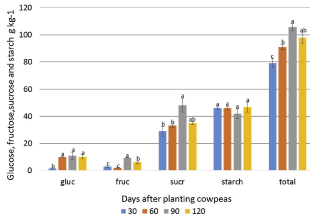
Fig. 2. Glucose (gluc), fructose (fruc), sucrose (suc) and starch concentrations and their totals in cowpea leaves harvested 30, 60, 90 and 120 d after planting. The data is from field experiment August to November 2016. The values represent means \pm standard error. Means labeled with the same letters within each sugar were not significantly different at p < 0.05 using Tukey's test ( n = 6 ).
