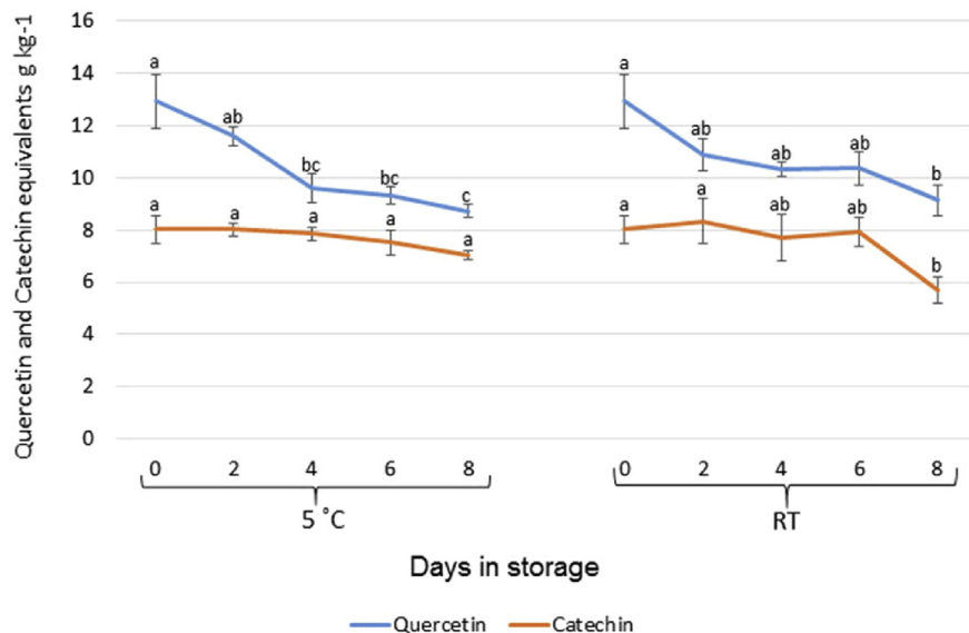
Fig. 7. Flavonoids (quercetin and catechin equivalents) in Cowpeas leaves harvested at 60 d after planting and stored at 5 °C and RT for 0, 2, 4, 6 and 8 d. The values represent means \pm standard error. Means labeled with the same letters within a metabolite were not significantly different at p < 0.05 using Tukey's test ( n = 6 ).
