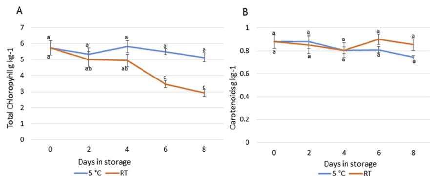
Fig. 13. A = Chlorophyll and B = carotenoid ( \text{g kg}^{-1} ) concentration in cowpea leaves harvested at 60 d after planting and stored at 5 °C and RT for 0, 2, 4, 6 and 8 d. The values represent means \pm standard error. Means labeled with the same letters within a group and storage condition were not significantly different at p < 0.05 using Tukey's test ( n = 6 ).
