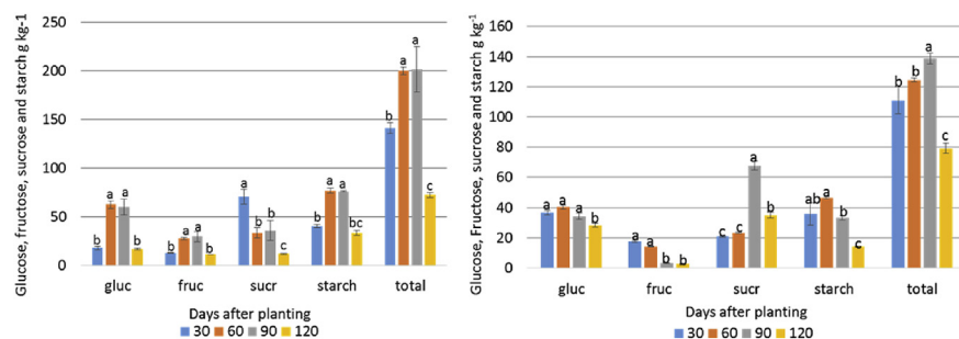
Fig. 3. A = Field experiments February to May 2015 and B = Field experiments November 2015 to February 2016: Glucose (gluc), fructose (fruc), sucrose (suc) and starch concentrations and their totals in cowpea leaves harvested 30, 60, 90 and 120 d after planting. The values represent means \pm standard error. Means labeled with the same letters within each sugar were not significantly different at p < 0.05 using Tukey's test ( n = 6 ).
