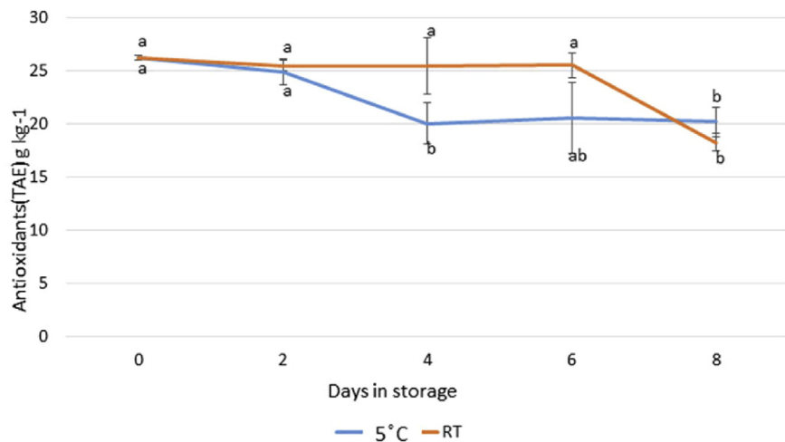
Fig. 11. Antioxidants (TEA) content in cowpeas leaves harvested at 60 d after planting and stored at 5 °C and RT for 0, 2, 4, 6 and 8 d. The values represent means \pm standard error. Means labeled with the same letters within a metabolite were not significantly different at p < 0.05 using Tukey's test ( n = 6 ).
