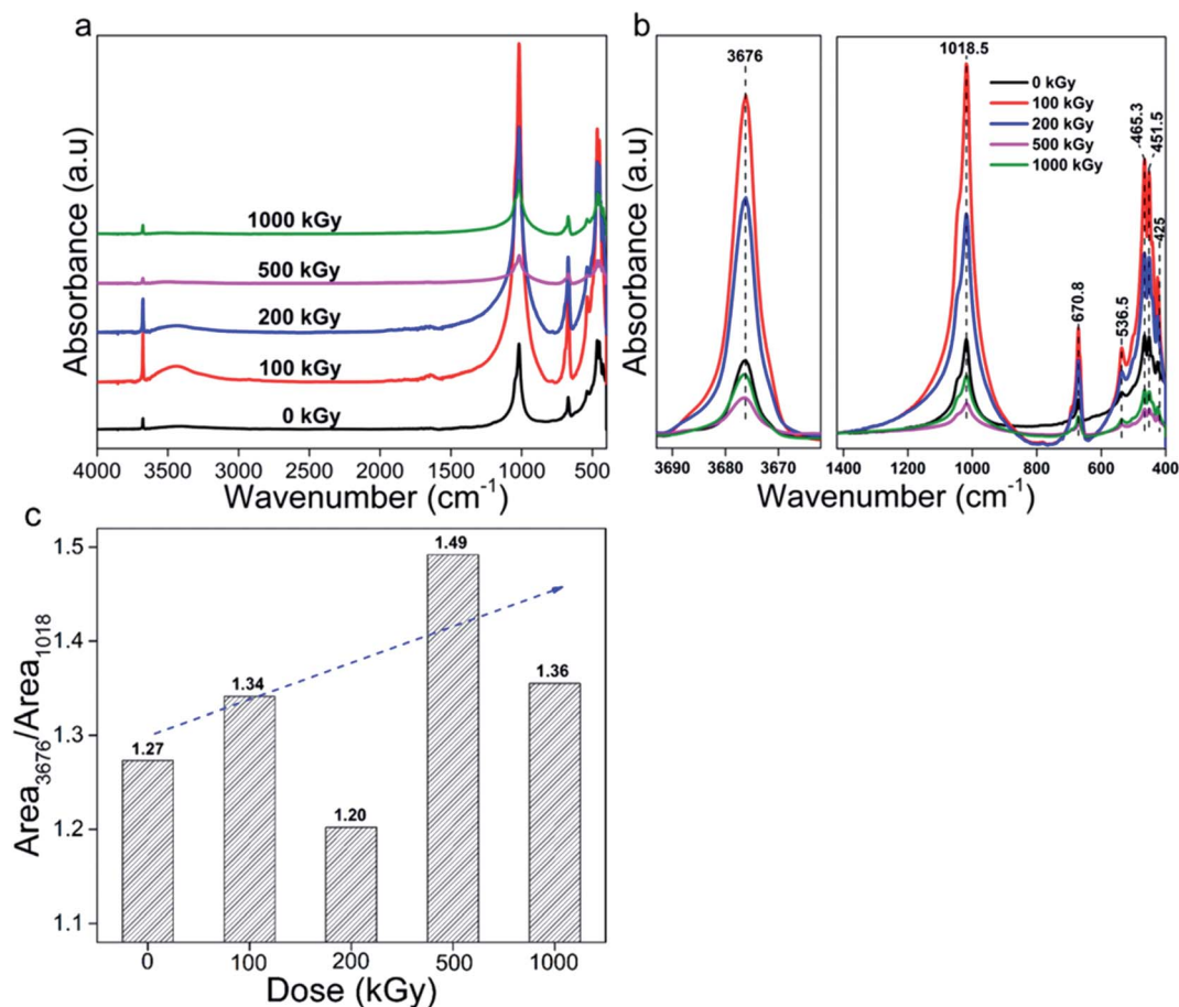
Fig. 5 FT-IR spectra of talc under EB irradiation with a dose of up to 1000 kGy: (a) complete; (b) refined. (c) Ratio of Mg–H to Si–O–Si vibration.
