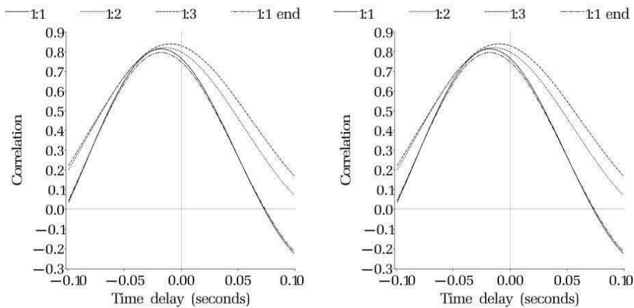
Figure 2 Time delays and inflation ratios. Time delays in couples of group 1 - left and group 2 - right, showing the relative delay for 1:1 (continuous line), 1:2 (dotted line), 1:3 (dashed line) and 1:1-end (intermittent dashed-dotted line) IABP inflation ratio.
