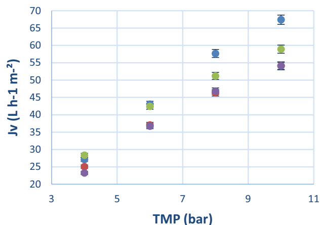
Figure 4. Effects of concentrations on permeate flux ( J_v ) as a function of transmembrane pressure (TMP). (●) 1.51 g L -1 , (●) 2.43 g L -1 , (●) 5.19 g L -1 , (●) 10.71 g L -1 .
