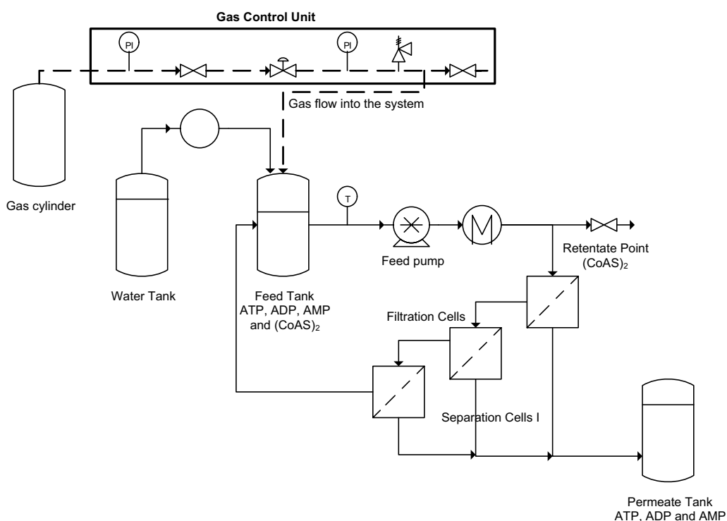
Figure 5. Experimental filtration set-up used for diafiltration experiments.
