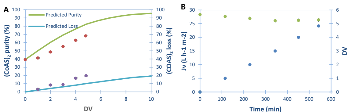
Figure 6. (A) Evolution of (CoAS) 2 purity (●) and loss (●) as a function of diafiltration volume (DV) during dia-ultrafiltration process with 5.19 g L -1 solution. (B) Evolution of permeate flux (Jv) (●) and diafiltration volume (DV) (●) as a function of time, with 5.19 g L -1 solution.
