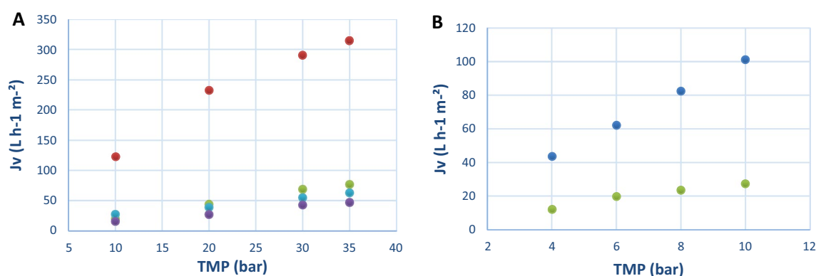
Figure 2. Effect of pressure (TMP) on permeate flux ( J_v ) for membranes screened with model solution. (A) (●) NP010, (●) GE, (●) 7450, (●) 7470 PHT. (B) (●) GK, (●) GR95PP.
