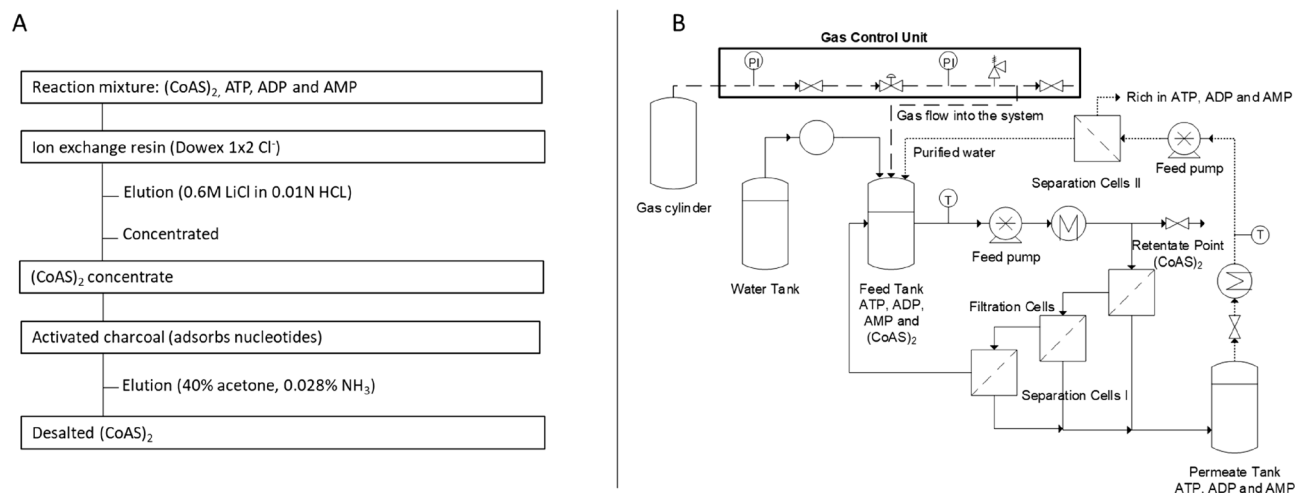
Figure 7. (A) Purification of (\text{CoAS})_2 through chromatography-charcoal adsorption/desorption strategy. (B) Purification of (\text{CoAS})_2 through cross-flow dia-filtration strategy.
