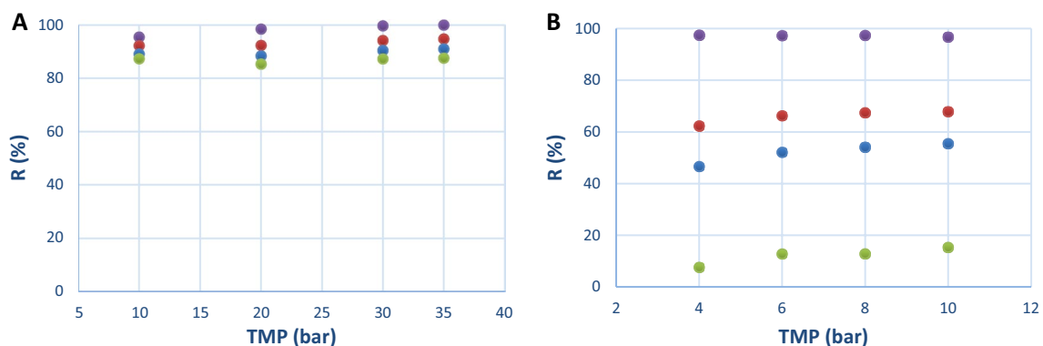
Figure 3. Effect of pressure (TMP) on the compounds' retention for (A) NP010 and (B) GK membranes with model solution. (●) (CoAS) 2 , (●) ATP, (●) ADP, (●) AMP.
