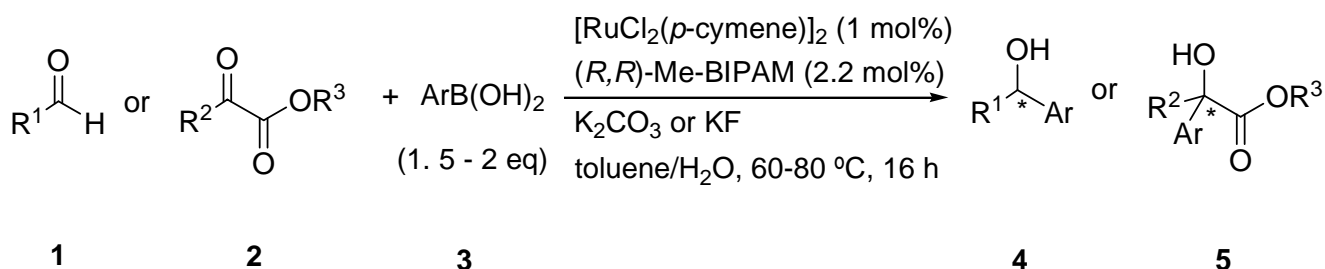
Scheme 1. Arylation of aliphatic aldehydes and \alpha -ketoesters.
