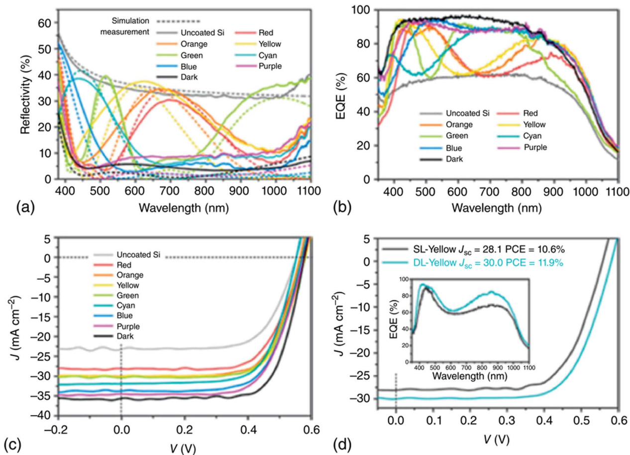
Fig. 10 (a) Modeled (dash lines) and observed (solid lines) reflection spectra of DL-MgF 2 /ZnS-coated G/Si heterojunction SCs (b) EQE spectra of the uncoated and G/Si SCs with various structural colors, (c) J - V spectra of the devices with various structural colors. J - V spectra of the devices without coating and with enhanced anti-reflection coating were also indicated for comparison, (d) contrast of the J - V and EQE (inset) among SL-ZnS-coated and DL-MgF 2 /ZnS-coated G/Si devices. (a)–(d) Have been reproduced from ref. 99 with permission from Elsevier.
