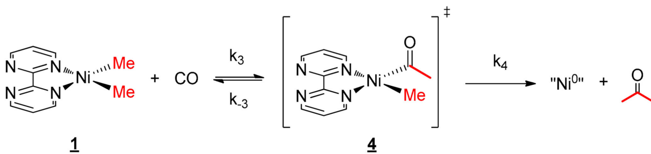
Scheme 4. Mechanism for the reaction of 1 with CO.
