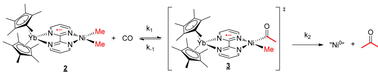
Scheme 3. Mechanism for the reaction of 2 with CO.
