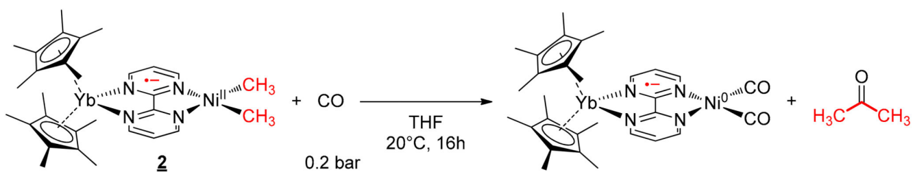
Scheme 2. Reactivity of 2 with carbon monoxide.
