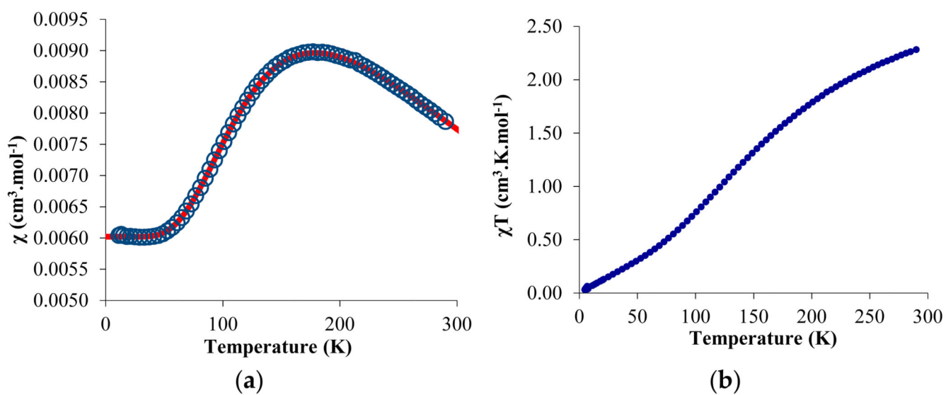
Figure 3. Solid-state temperature-dependent magnetic data at 0.5 T: (a) plot of \chi versus T and of (b) \chi T versus T. The solid line represents the fit of the magnetic data (see text).
