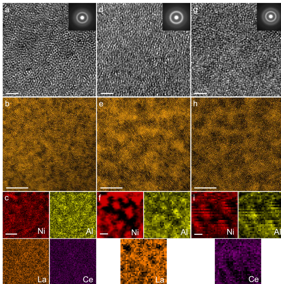
Fig. 3 The atomic structures and corresponding elemental distributions of the La(Ce)NiAl system. a, d, g HRTEM images presenting uniform mazelike patterns for the as-cast LaCe-HEMG, \text{La}_{55}\text{Ni}_{20}\text{Al}_{25} , and \text{Ce}_{55}\text{Ni}_{20}\text{Al}_{25} , respectively, the corresponding SAED patterns (insets) demonstrating the typical amorphous structures. Scale bars: 2 nm. b, e, h HAADF-STEM images of LaCe-HEMG, \text{La}_{55}\text{Ni}_{20}\text{Al}_{25} and \text{Ce}_{55}\text{Ni}_{20}\text{Al}_{25} , respectively. Scale bars: 5 nm. c, f, i Corresponding EDS chemical mappings for LaCe-HEMG, \text{La}_{55}\text{Ni}_{20}\text{Al}_{25} and \text{Ce}_{55}\text{Ni}_{20}\text{Al}_{25} , respectively. LaCe-HEMG exhibits relatively homogeneous elemental distributions. Scale bars: 5 nm.
