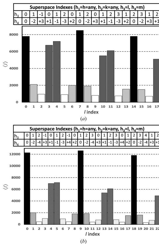
Figure 2 Average reflection intensities as a function of the l index. The superspace indexing of the same average reflection intensities ( h_3 and h_4 ) is shown for (a) PDB entry 4n3e and (b) PDB entry 6sjj. These charts were adapted from Sliwiak et al. (2015) and Smietanska et al. (2020).
