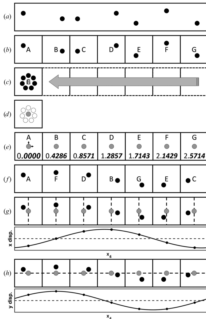
Figure 5 The process of converting a supercell into its subspace representation: (a) the supercell, (b) partitioning of the supercell into the basic cell, (c) translation of all of the basic cells to overlap with the first basic cell, (d) calculation of the average positions from the translated positions of related elements, (e) using the average position in each basic cell to determine \mathbf{x}_4 , (f) sorting the basic cells by fractional \mathbf{x}_4 , (g) determining horizontal displacements from the average as a function along \mathbf{x}_4 and (h) determining vertical displacements from the average as a function of \mathbf{x}_4 .
