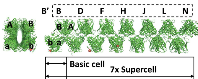
Figure 4 The superstructure of PDB entry 4n3e with views looking down and along the structure. The supercell is a sevenfold expansion in the c direction. Chains in the first basic cell (a, b, A and B) use a notation with a prime to denote all related chains in subsequent basic cells; for example, B' refers to chains B, D, F, H, J, L and N. The PDB entry 6sjj supercell looks similar but has two additional basic cells and uses a slightly different naming scheme for the chains.
