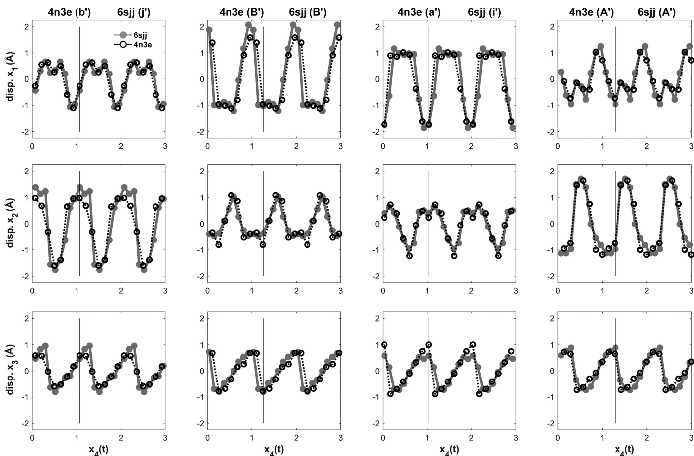
Figure 8 AMF approximations using the average centre of mass for each of the four chains in the ASUs for PDB entry 4n3e ( \mathbf{q} = 3/7\mathbf{a}_3^* ) and PDB entry 6sjj ( \mathbf{q} = 4/9\mathbf{a}_3^* ) in the x_1 , x_2 and x_3 directions as a function of x_4 .
