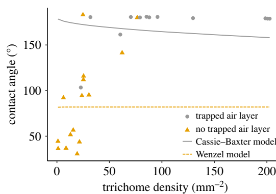
Figure 6. Contact angle of water droplets on leaves with varying trichome density replotted with permission from [133], copyright © 2006 John Wiley and Sons. Coloured circles and triangles indicate whether a trapped air layer was experimentally observed or not. Solid and dashed lines indicate approximate Cassie–Baxter and Wenzel model predictions based on assumption that trichomes are cylinders of 0.1 \times 0.42 mm and with a reference contact angle of 82^\circ .
