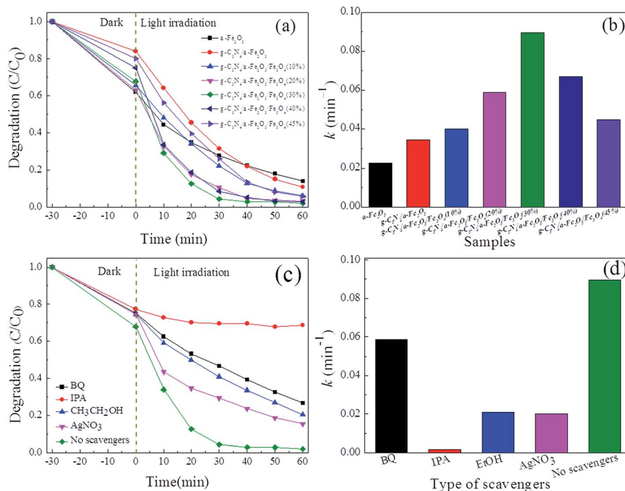
Fig. 5 (a) Degradation rate and (b) kinetic constant of all samples, (c) degradation rate and (d) kinetic constant of g\text{-C}_3\text{N}_4/\alpha\text{-Fe}_2\text{O}_3/\text{Fe}_3\text{O}_4 (30%) samples with different scavengers.
