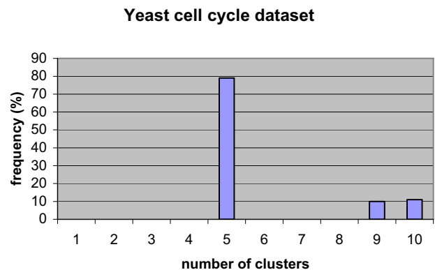
Figure 3 Histogram of determined optimal number of clusters in ten-fold cross-validation on yeast cell cycle data set.
