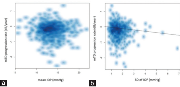
Figure 4. (a) The relationship between the mTD progression rate and mean IOP. There was no significant relationship between the mTD progression rate and mean IOP ( P = 0.32 , linear mixed model). (b) The relationship between the mTD progression rate and SD of IOP ( P = 0.011 , linear mixed model). IOP: intraocular pressure; mTD: mean total deviation; SD: standard deviation. (From Fujino et al Invest Ophthalmol Vis Sci 2016).
