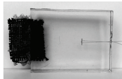
FIGURE 3: Specimen made of ballistic gelatin with casted-in PF anchor. The fabric on the left side of the specimen is used for proper clamping in the tensile testing machine.
