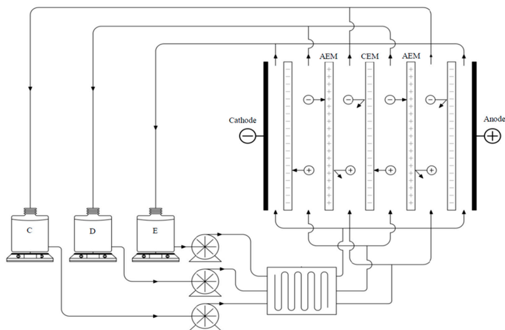
Figure 2. The experimental arrangement used for the electrodesalination (ED) experiments ((C = concentrate, D = diluate, E = electrolyte, CEM = cation exchange membrane, AEM = anion exchange membrane).
