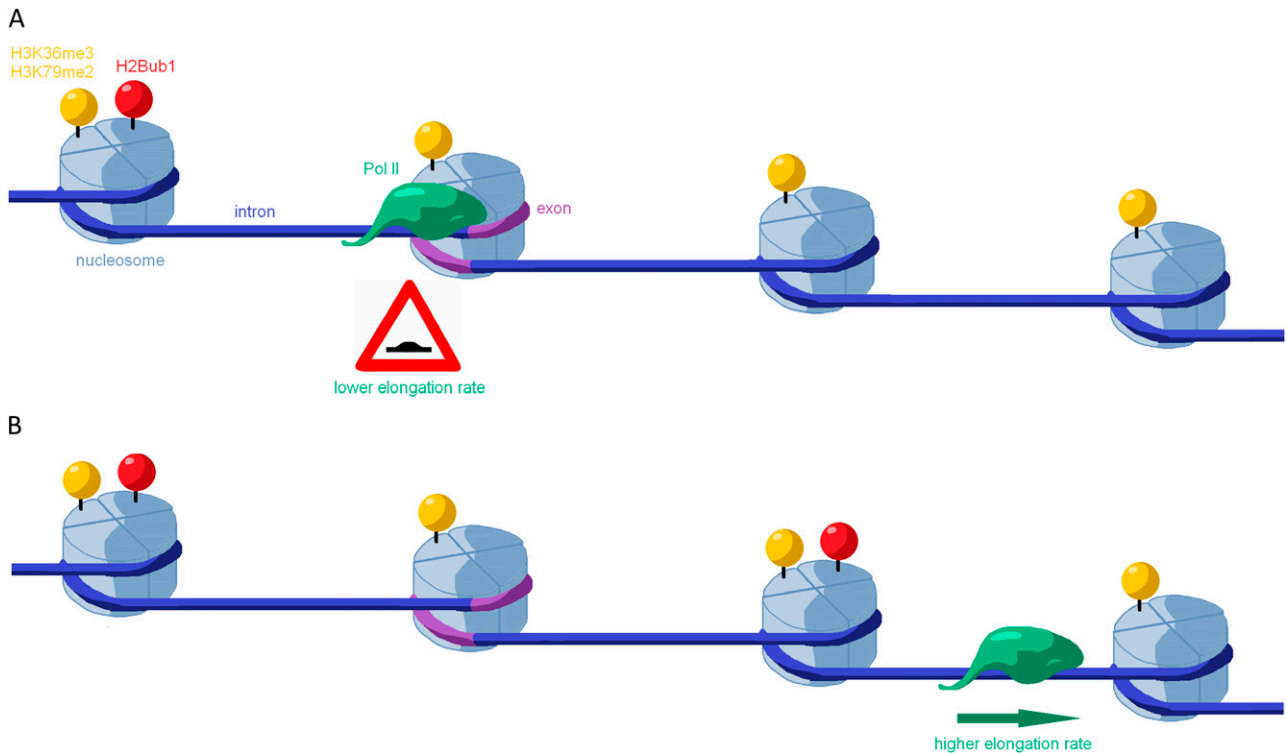
Figure 7. Model depicting the coupling between H2Bub1 distribution within gene bodies and Pol II elongation rate. H2Bub1 distribution is highly coupled to Pol II elongation within transcribed regions. While H3K36me3 and H3K79me2 do not mirror Pol II kinetics at this time resolution, H2B is monoubiquitylated as Pol II progresses along the gene (A to B). Furthermore, Pol II pausing or a slower elongation rate at exons compared to flanking introns is coupled with lower H2Bub1 levels.
