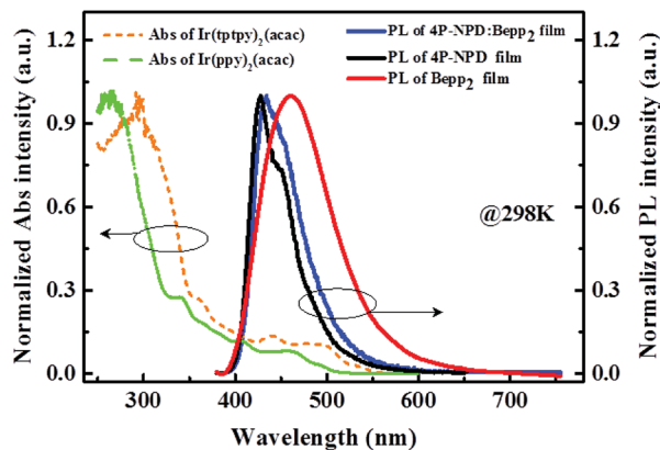
Fig. 6 Normalized absorption spectra of \text{Ir}(\text{ppy})_2(\text{acac}) and \text{Ir}(\text{tptpy})_2(\text{acac}) measured in \text{CH}_2\text{Cl}_2 solvent as well as photoluminescence spectra of pure 4P-NPD, pure Bepp 2 , and 4P-NPD : Bepp 2 (2 : 1) mixture solid films.
