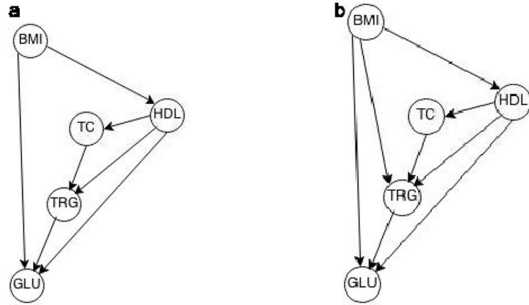
Figure 2. a. Estimated causal structure African-American (3856 individuals) b. Estimated causal structure European-American (10753 individuals).
