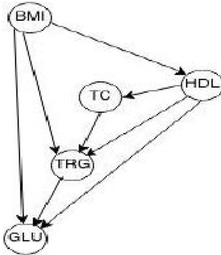
Figure 1. The estimated causal graph across the entire sample set.
